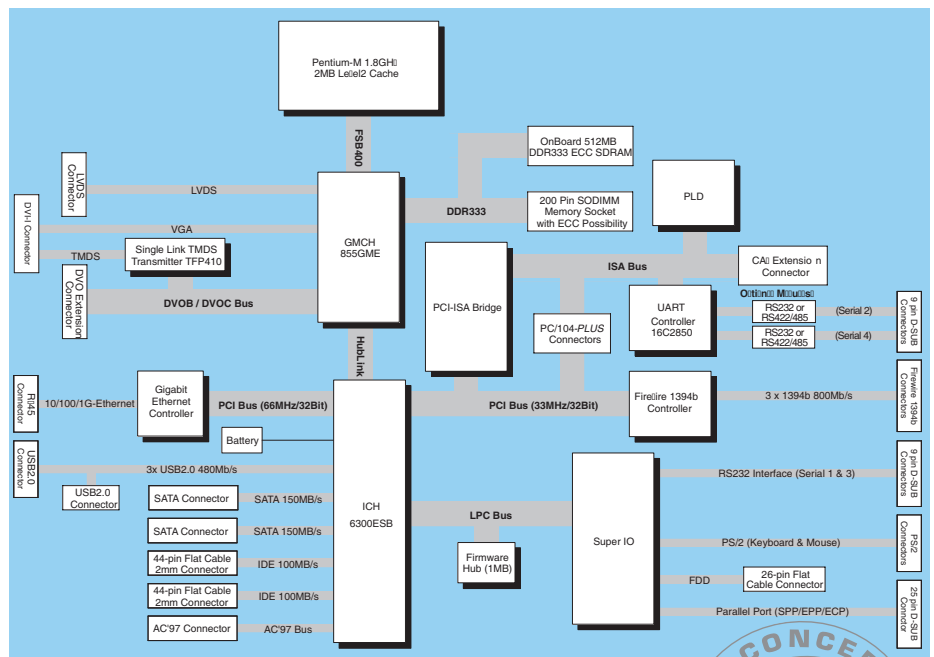
PIP11 hardened Industrial PC in rugged aluminum housing
